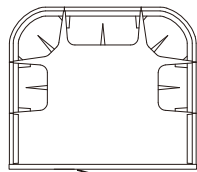
WS-206ST(P5) Size:2200X1906X2100mm
