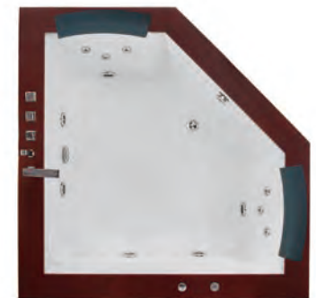
WS-0503 Size: 1800x1800x680mm Size: 1500x1500x680mm
