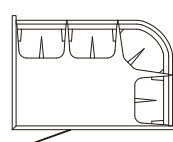
WS-201ST-W4(L/R) Size: 1345X1945X2100mm
