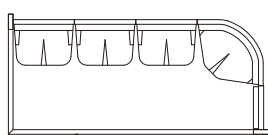
WS-200ST-W4(L/R) Size: 1175X2545X2100mm
