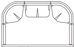
WS-205ST(P3) Size:2050X1306X2100mm
