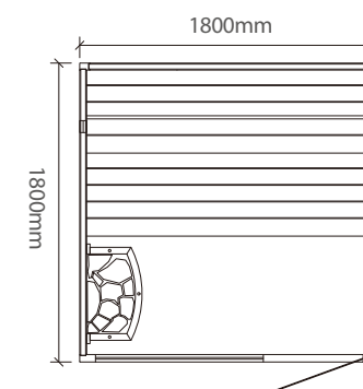
WS-CC02 Size:1800x1800x2100mm
